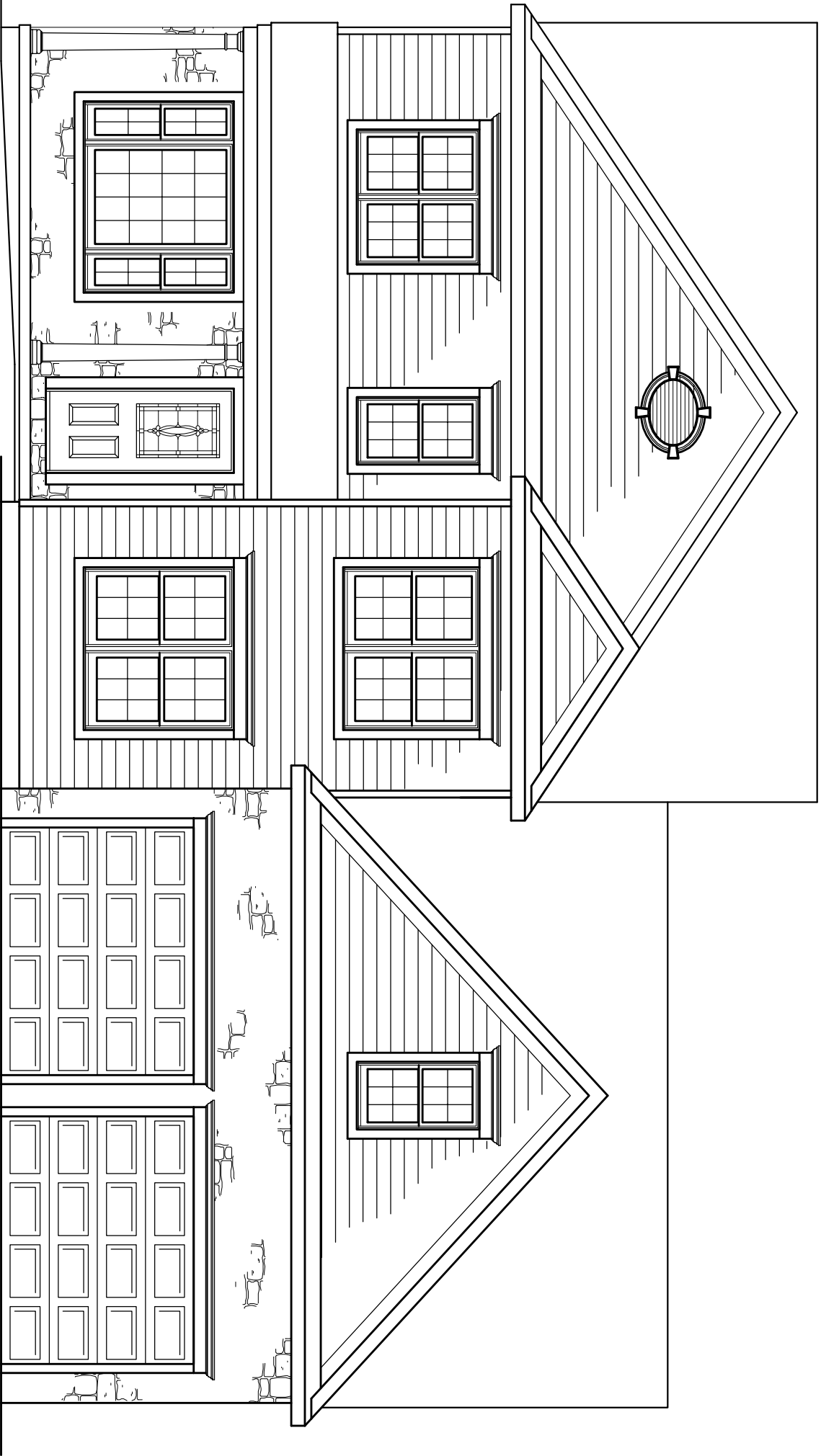
FRONT ELEVATION
