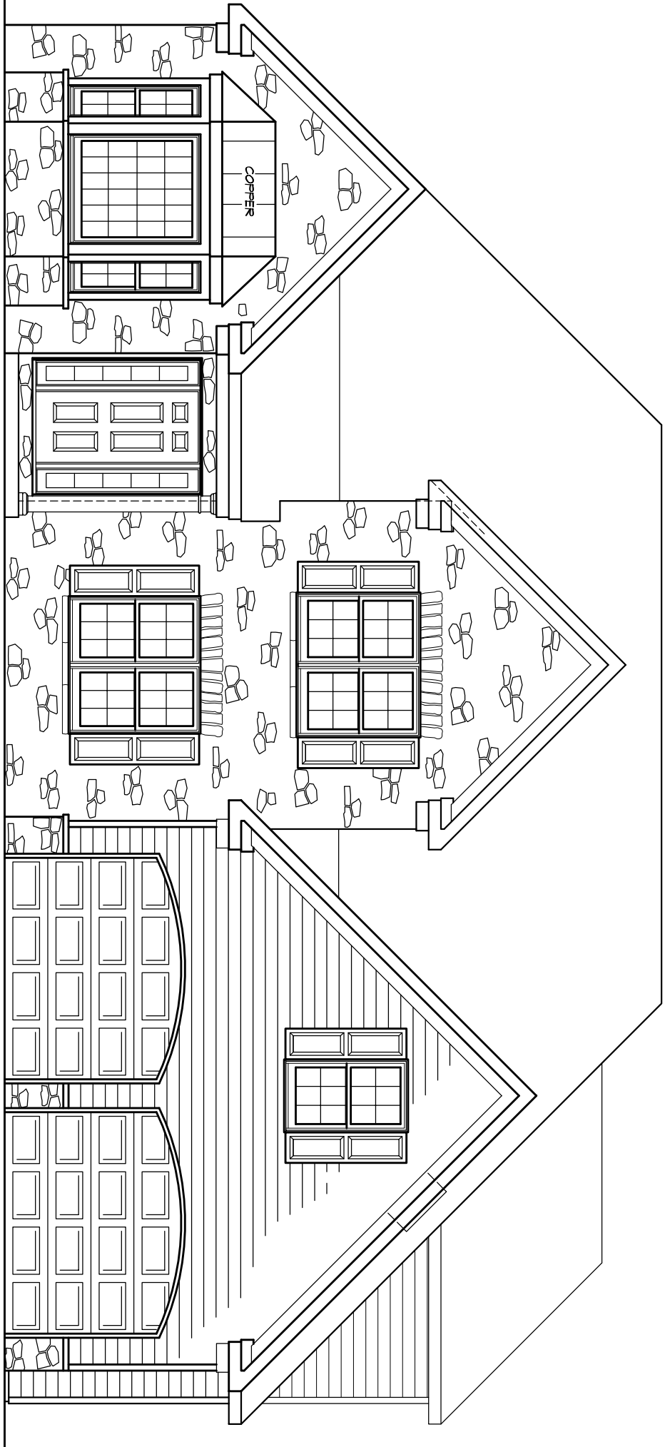
FRONT ELEVATION
